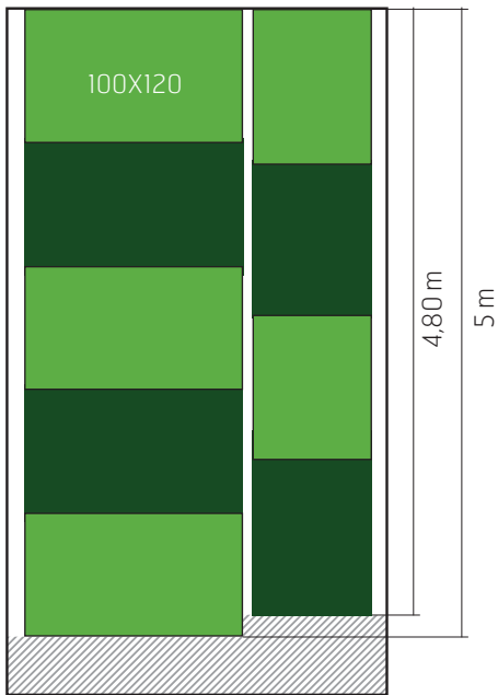
20' REEFER = 9 PALLETS
